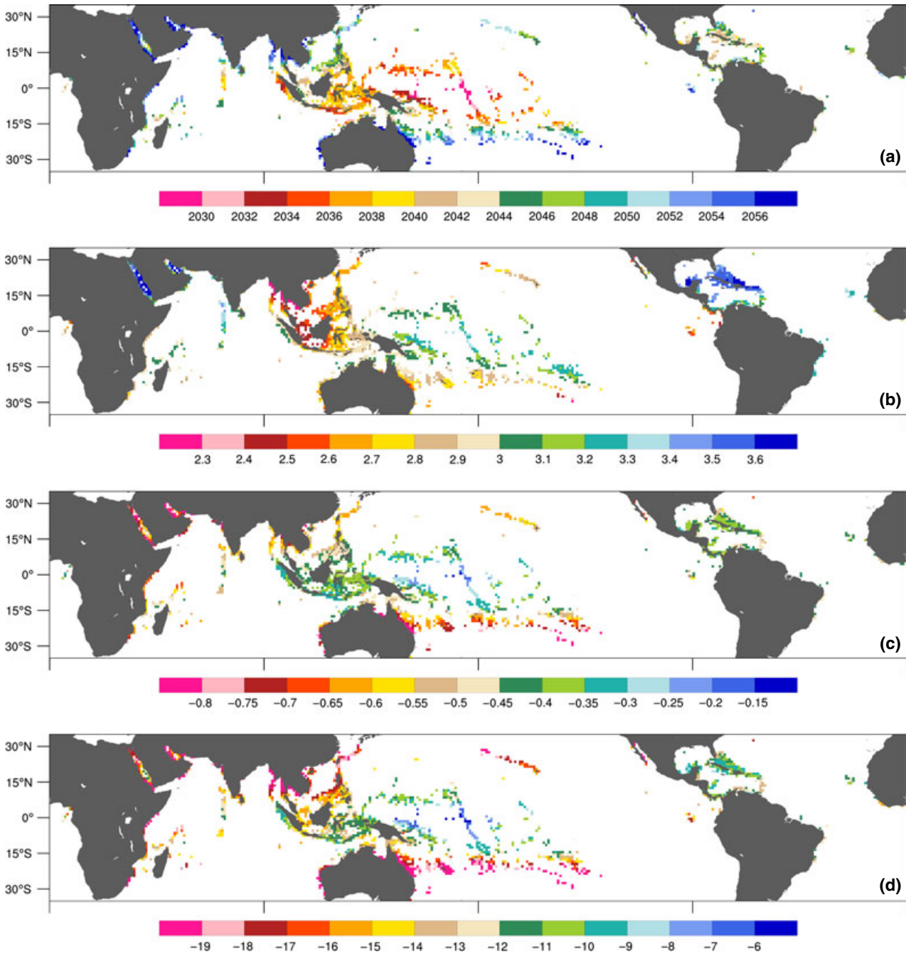
Fig. 1 Projections for coral reefs based on multimodel ensembles forced with RCP8.5 for the year reefs start to experience 8 DHWs annually (a). \Omega_{arag} in the year in (a) is shown in (b) and the reduction in \Omega_{arag} from 2006 until the year shown in (a) is shown in (c). The data shown in (c) are expressed as a percentage change from 2006 values in (d).
